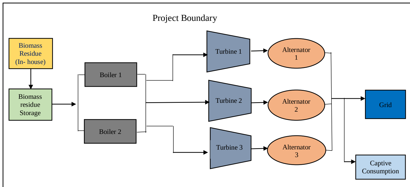
Figure 5: Schematic representation of project boundary
