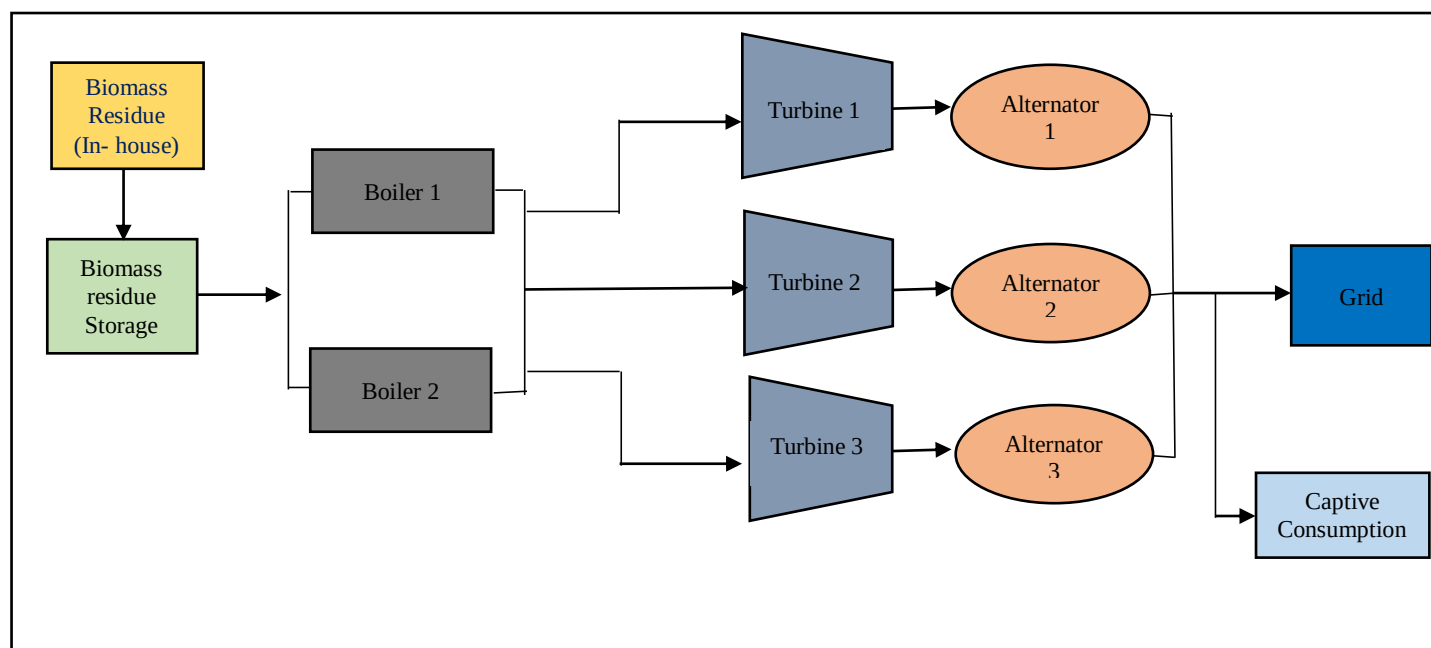
Figure 2: Schematic representation of the process flow chart
